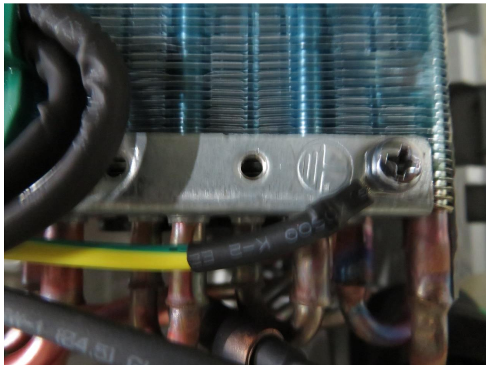
Earthing screws
