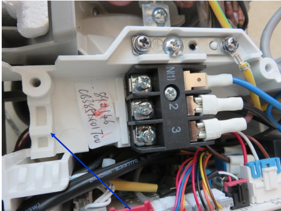
Cord anchorage
